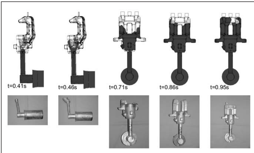
Figure 3: Comparison of interrupted filling tests
