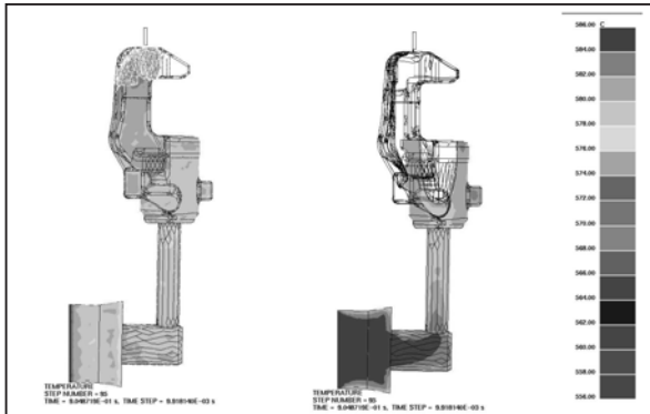
Figure 4: Temperature contour plot showing premature solidification
