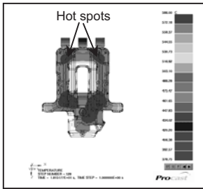
Figure 5: Areas of hot spots
