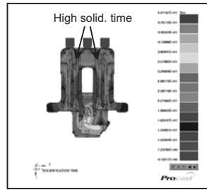
Figure 6: Solidification time
