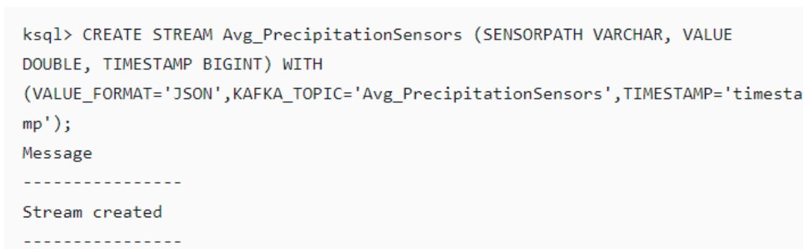
Figure 14. Creating topic in the Kafka broker through the terminal.
