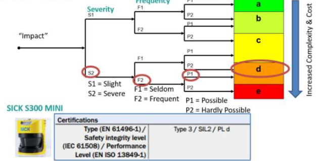
Figure 13 Risk assessment for "head-on collision" according to ISO 13849-1.
