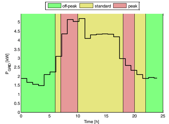
Fig. 3: Load exclusively supplied by the grid
