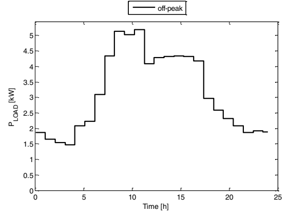
Fig. 2: Proposed domestic load profile [12]
