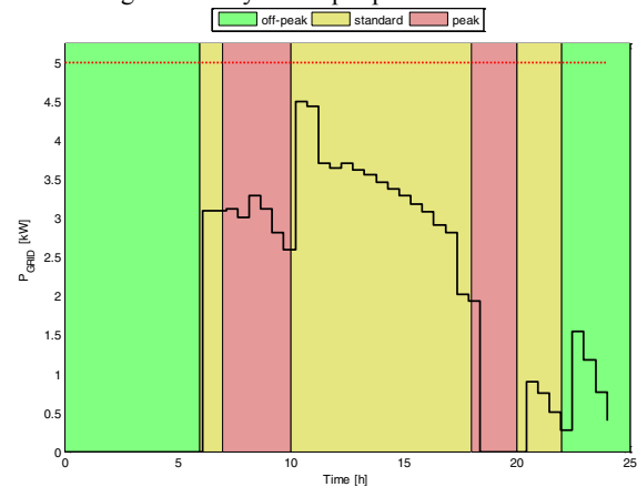
Fig. 7: Grid power to the load
