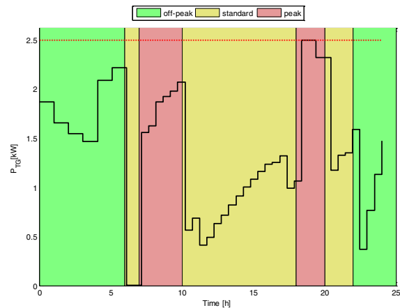
Fig. 6: Pico hydro output power to the load
