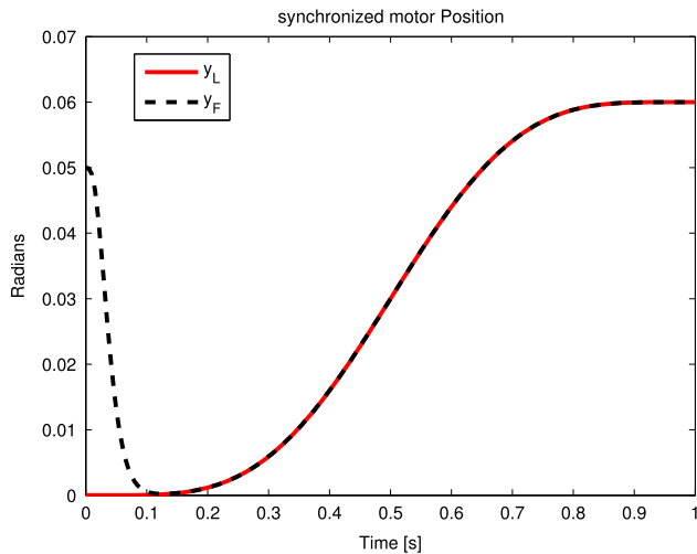
Fig. 7. Tip position of follower and leader robots in closed loop for flat output reference (case 1).
